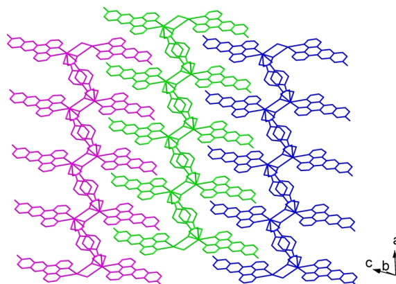
Fig. 3 (color online). Supramolecular layer structure of [Pb(1,4-chdc)(L)] (1) constructed by \pi - \pi interactions.
