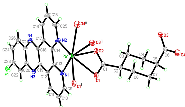
Fig. 1 (color online). The coordination environment of the Pb(II) atom in the molecular structure of [Pb(1,4-chdc)(L)] (1) in the crystal.
