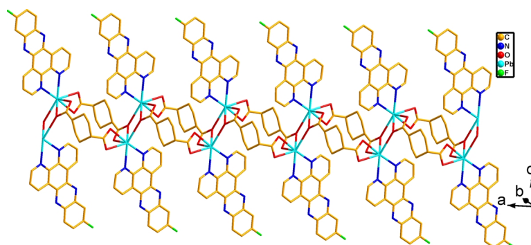
Fig. 2 (color online). View of the one-dimensional chain structure of crystalline [Pb(1,4-chdc)(L)] (1).
